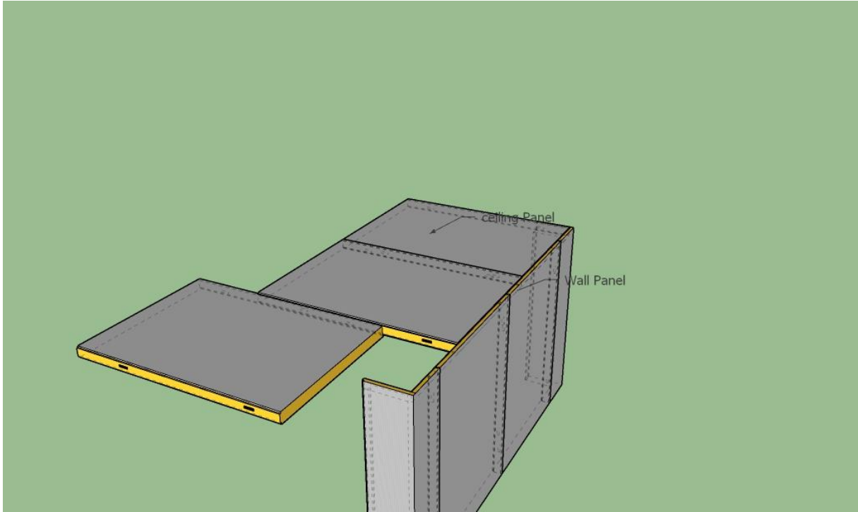
2 -) According to Wall panel ceiling panel installtion
