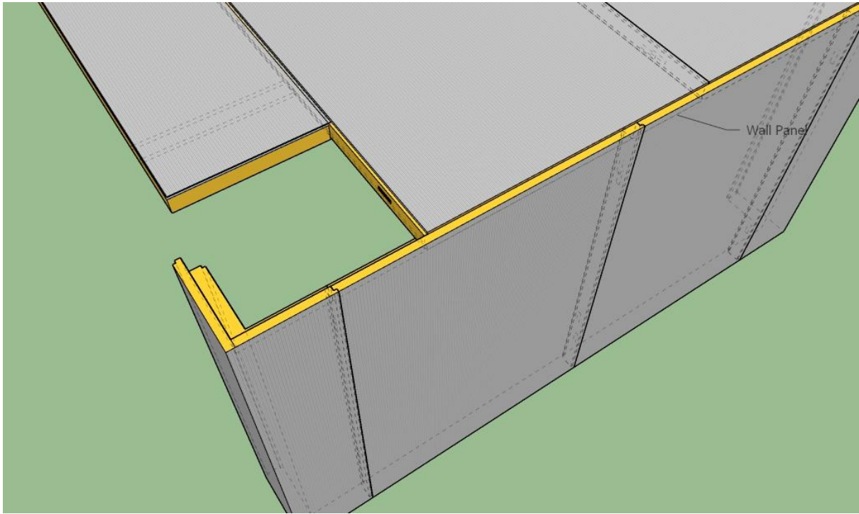
3-) According to ceiling panel last one need to cut necessary size
